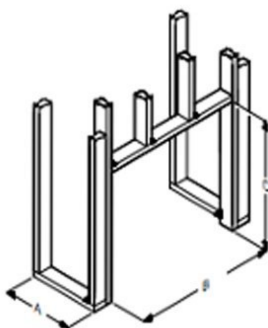
Rough-In Framing Dimensions
