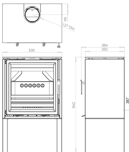
Ecostar 5 Wide Houtvak
