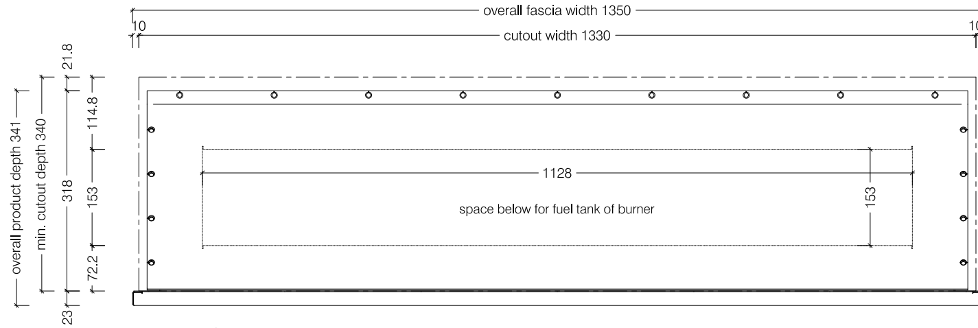
Top View
