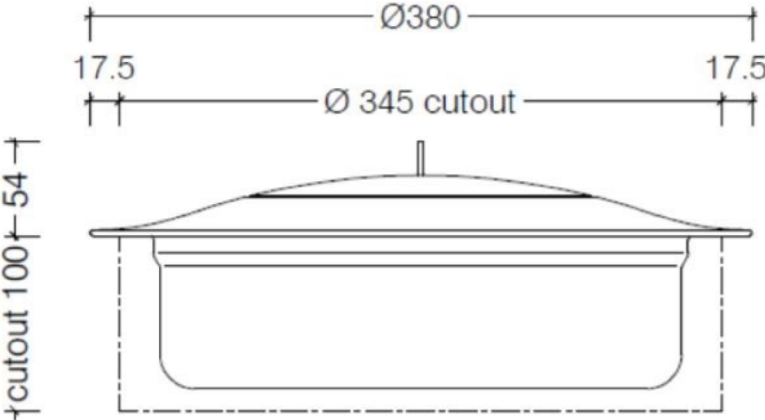
Side View
